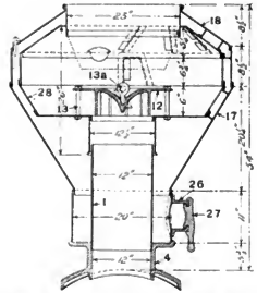
Figs. 474-475. Diamond Stack for Wood Burning Locomotive.
